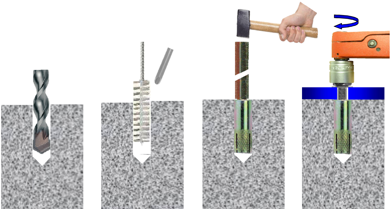
Drill correct diameter hole to correct depth
